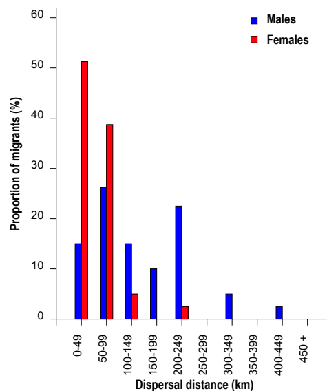
Fig. 2.12. Proportion of migrating lynxes and their migration distance (after Andersen et al. 2003).
