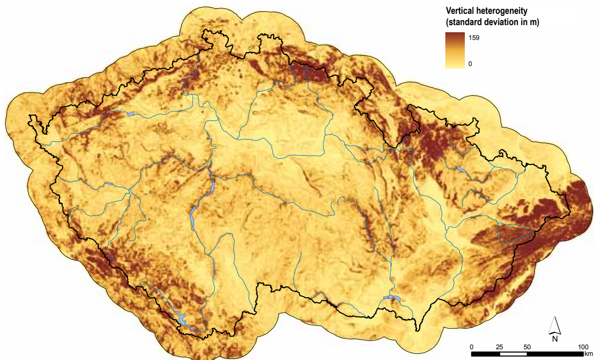
Fig. 4.3. Vertical heterogeneity (source: DEM SRTM 100 × 100 m 2009).
