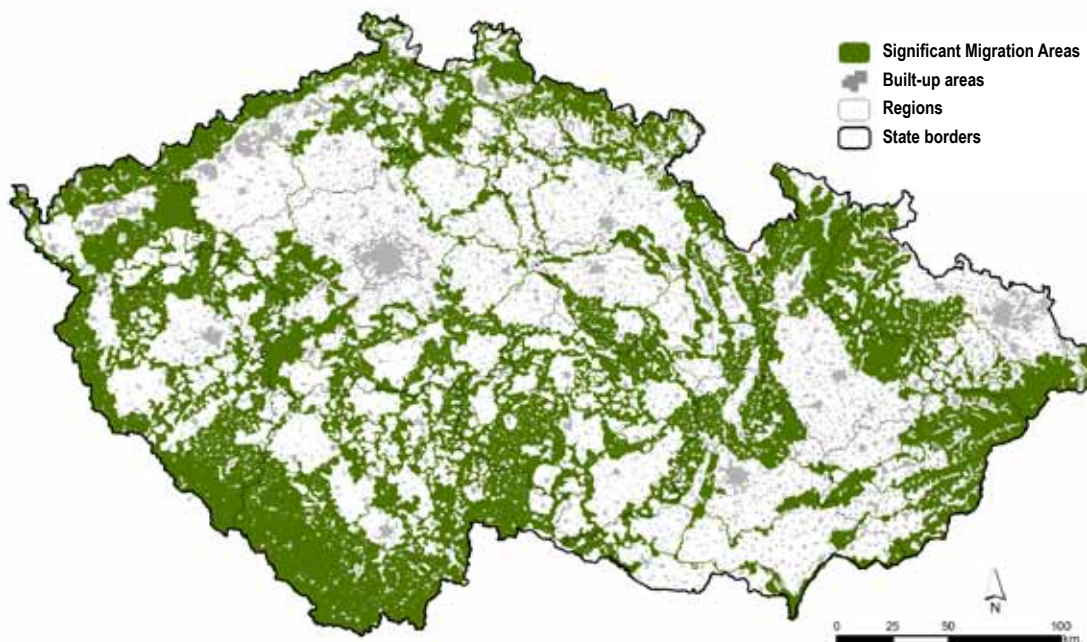
Fig. 6.1. Synoptic map of Significant Migration Areas.
