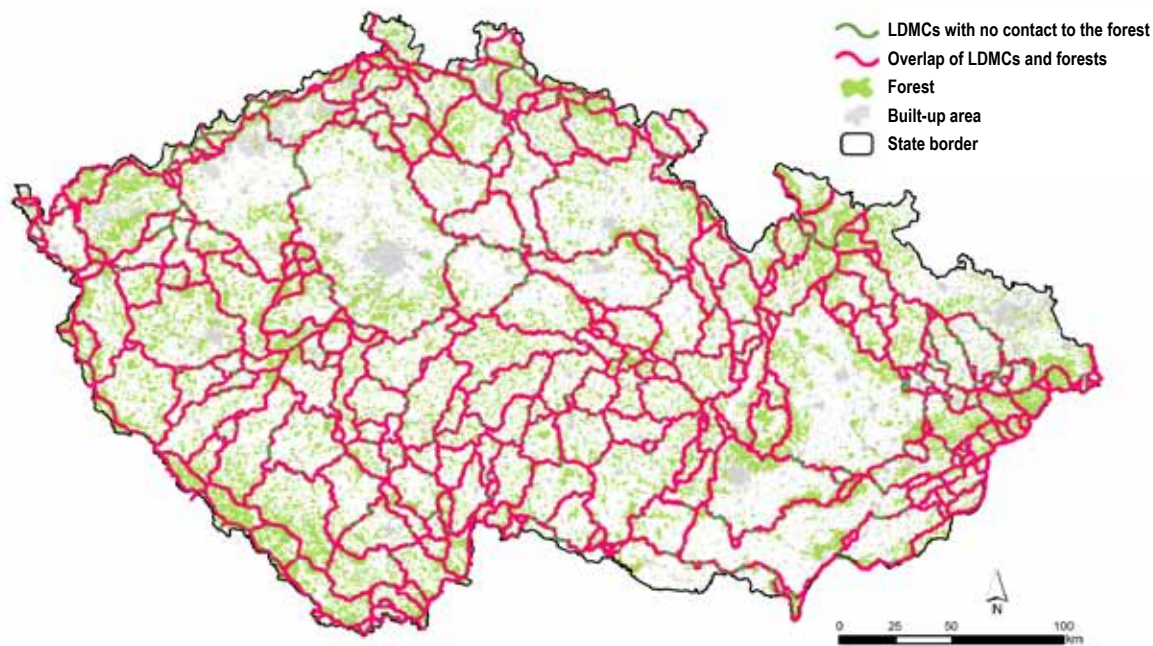
Fig. 7.9. LDMCs and the forest cover.
