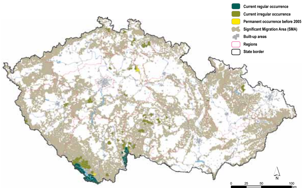
Fig. 6.5. Records of the Eurasian Elk supplied from the AOPK database and compared with SMAs.
