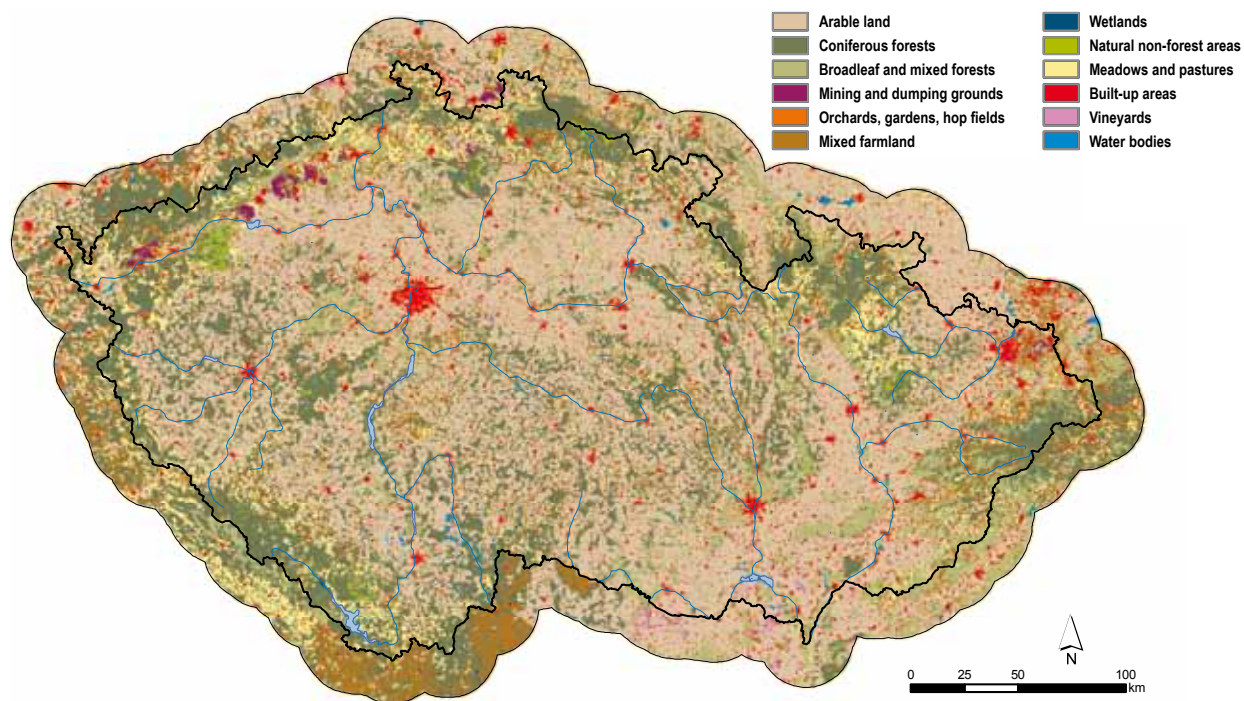
Fig. 4.4. Land cover – generalised classes (source: CORINE Land Cover 2006, EEA 2009).
