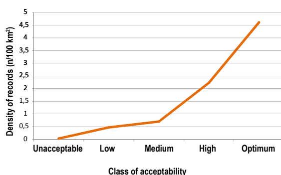
Fig. 5.8. Relation of the density of records and the level of acceptability of the given area – Eurasian Lynx; occurrence.
