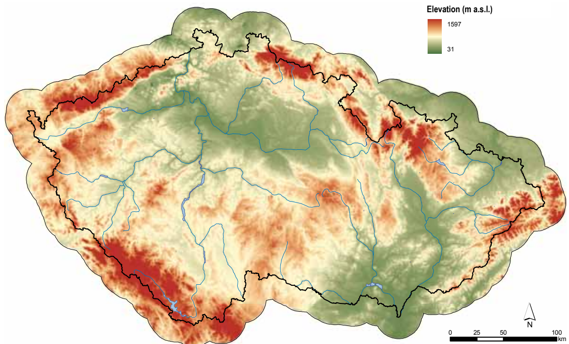
Fig. 4.2. Elevation (source: DEM SRTM 100 × 100 m 2009).
